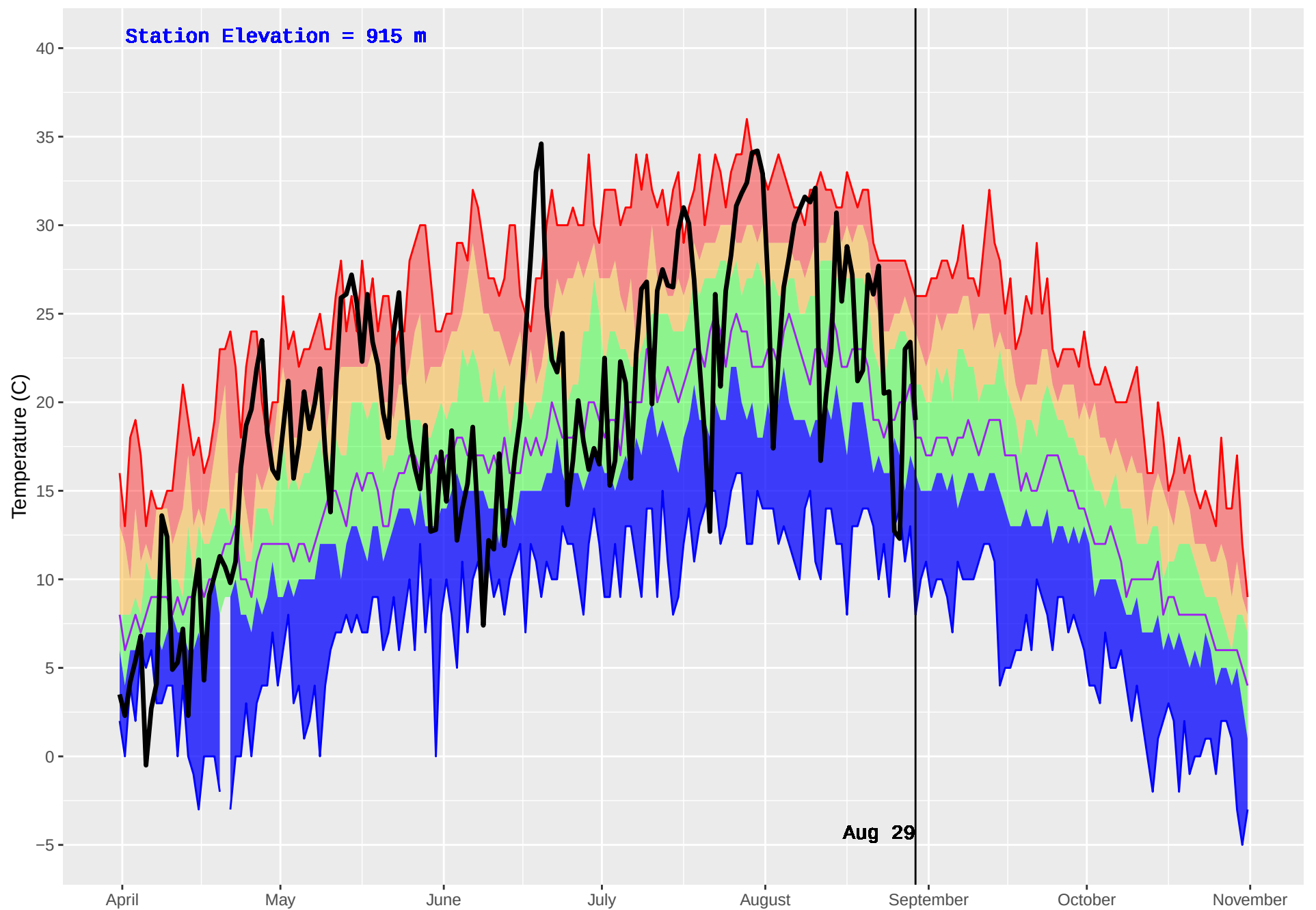
MIDDLE LAKE (226) : Historical (1989–2016) and Current (2018) Daily Temperature
